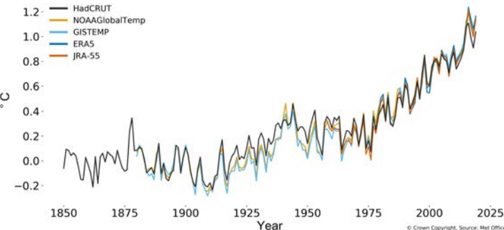
Global mean temperature difference from 1850-1900 (°C)
